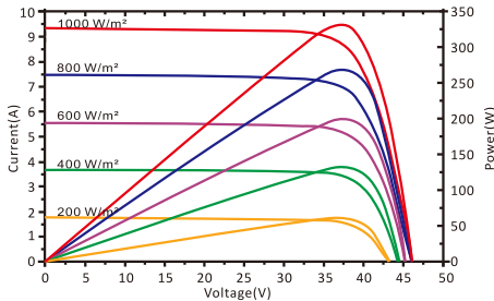
I-V characteristics at different irradiances
